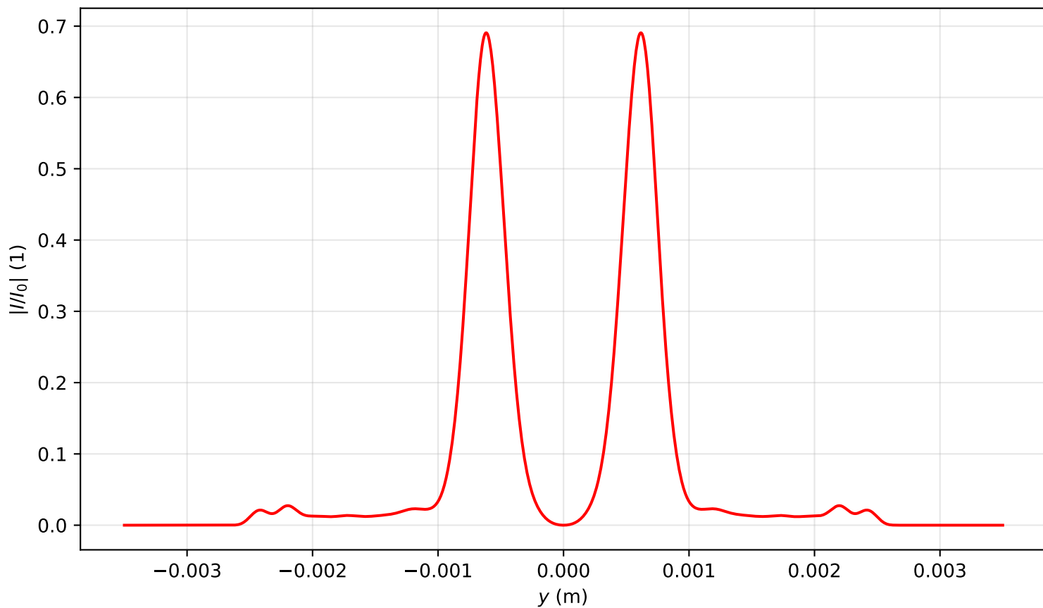
Intensity profile I(x=0, y, z=2.070)/I_0 , \text{Pin}=7.0\text{Pcr} , artificial time
